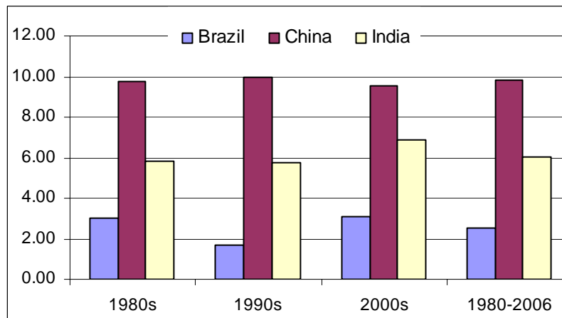
Figure 2: Average growth rates: Brazil, China and India (per cent)
